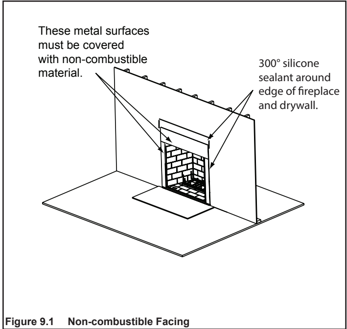
Figure 9.1 Non-combustible Facing
