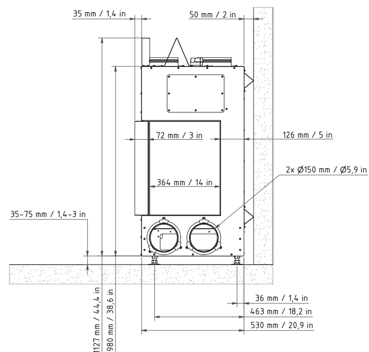
Side view 1:20
