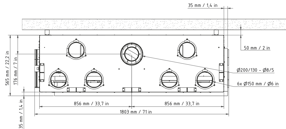
Side view 1:20
