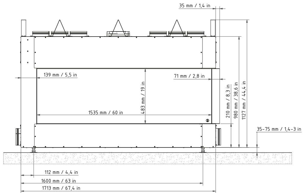
Top view 1:20
